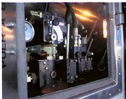
Electric Hydraulic Valve with manual levers
